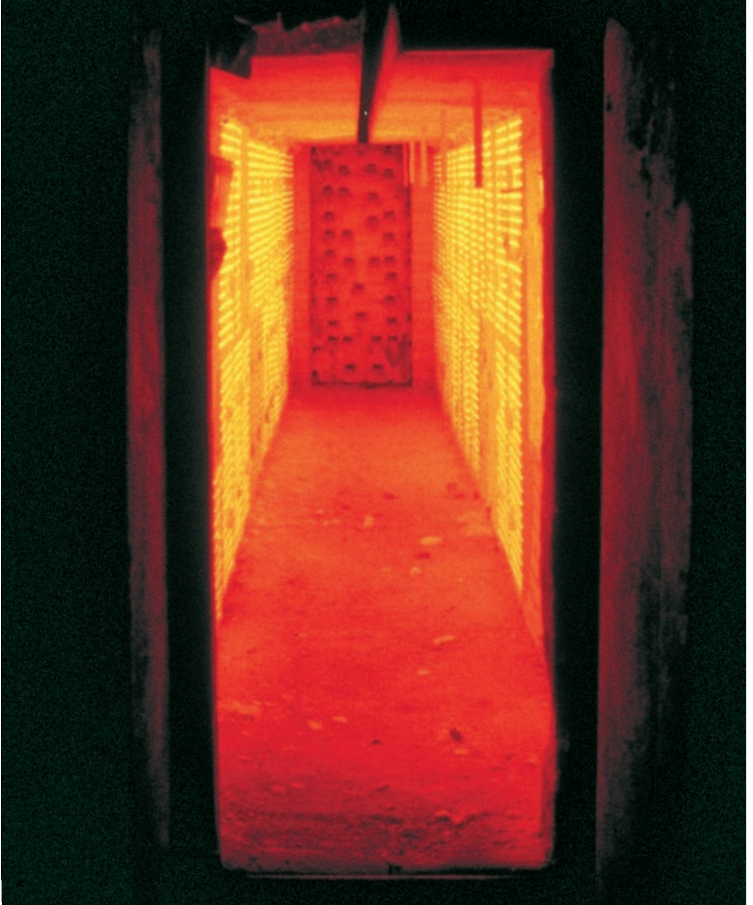
Fig. 19 Fibrothal modules in a suspended monorail furnace.
